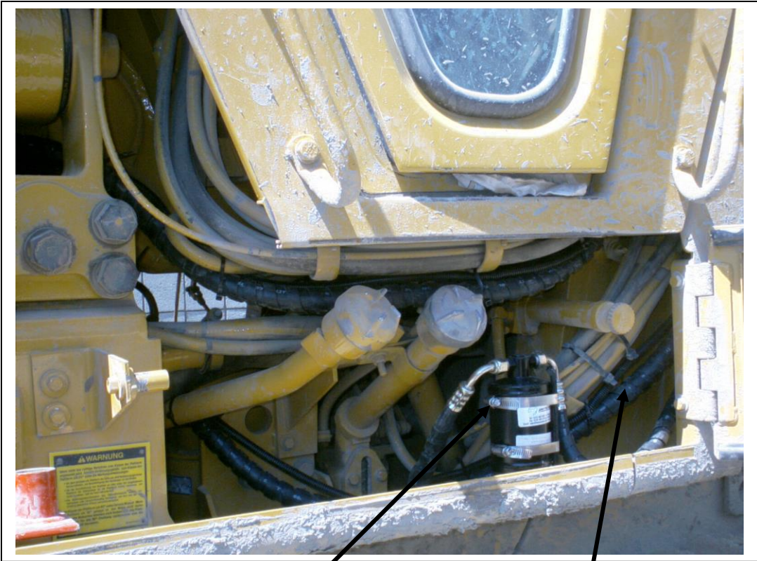
Receiver drier location
