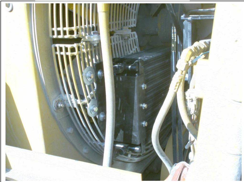
Right side of condenser mounted to fan screen
